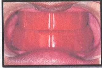
JAW RELATION
