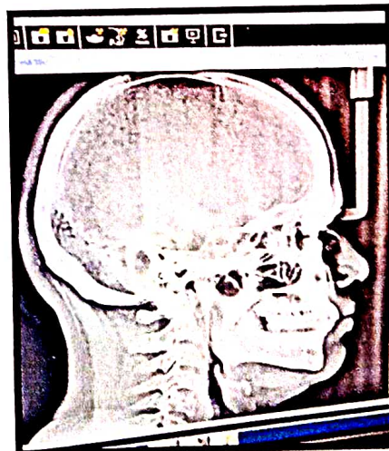
Morphometric softwares
